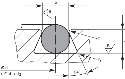
Dovetail gland
